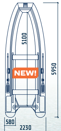
Solar-595 Super Jet Tunnel
