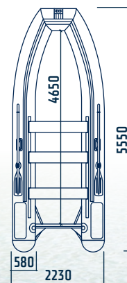
Solar-555 Super Jet Tunnel
