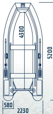
Solar-520 Super Jet Tunnel
